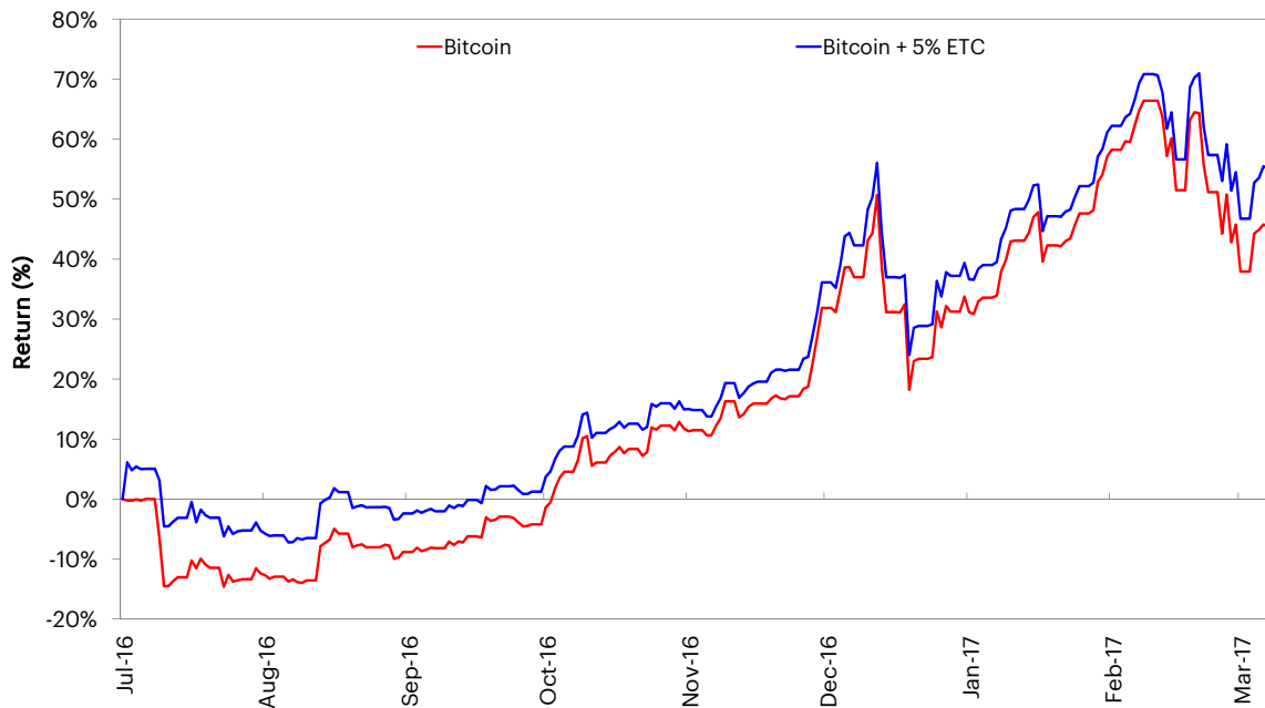
Hypothetical Simulated Portfolio Performance Cumulative (ln)
