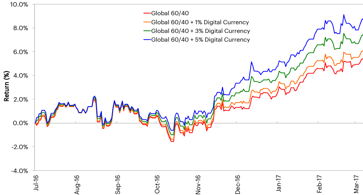
Hypothetical Simulated Portfolio Performance Cumulative (In)
